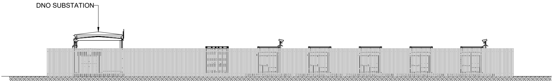
BATTERY ENERGY STORAGE SYSTEM (BESS) COMPOUND ELEVATION D
