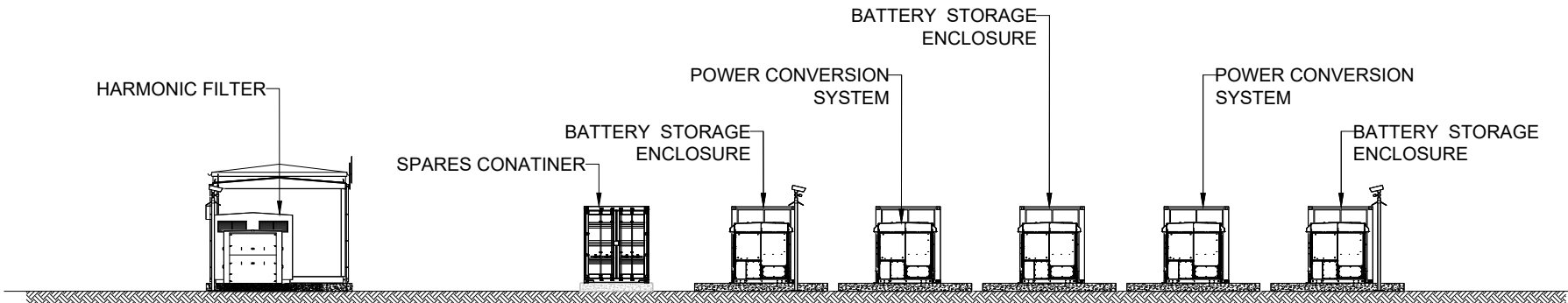
BATTERY ENERGY STORAGE SYSTEM (BESS) COMPOUND ELEVATION D
