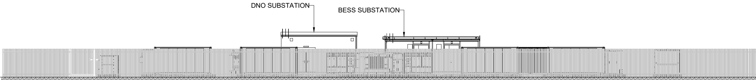
BATTERY ENERGY STORAGE SYSTEM (BESS) COMPOUND ELEVATION C (WITH PERIMETER FENCE)
