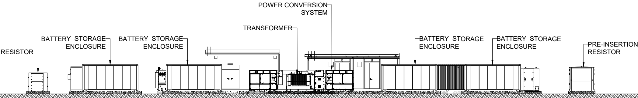
BATTERY ENERGY STORAGE SYSTEM (BESS) COMPOUND ELEVATION C
