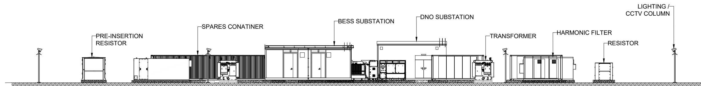
BATTERY ENERGY STORAGE SYSTEM (BESS) COMPOUND ELEVATION A
