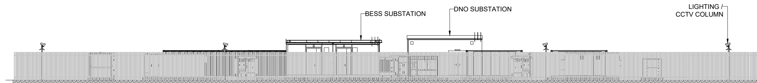
BATTERY ENERGY STORAGE SYSTEM (BESS) COMPOUND ELEVATION A (WITH PERIMETER FENCE)
