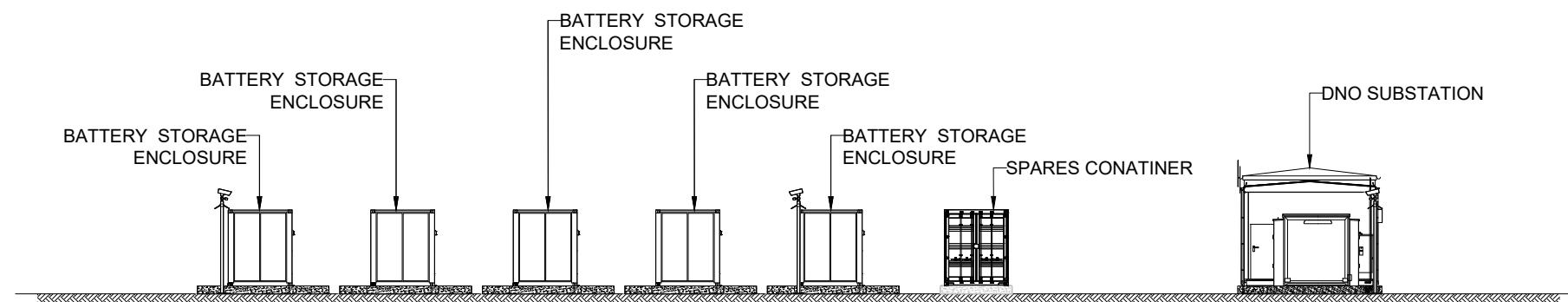
BATTERY ENERGY STORAGE SYSTEM (BESS) COMPOUND ELEVATION B
