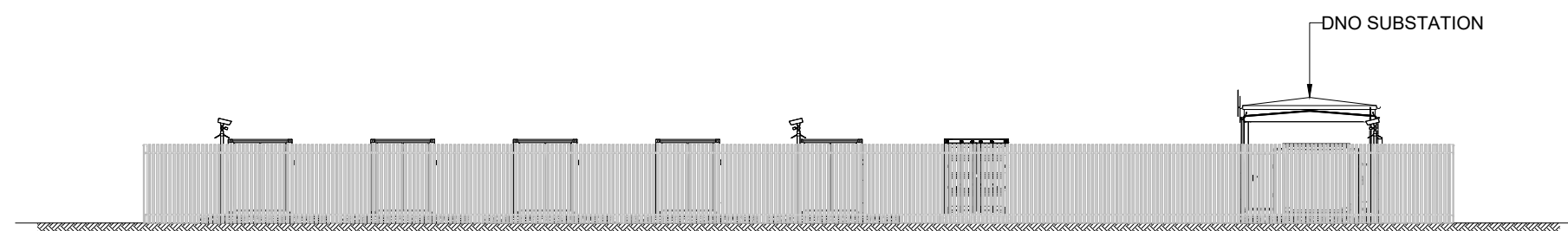
BATTERY ENERGY STORAGE SYSTEM (BESS) COMPOUND ELEVATION B
