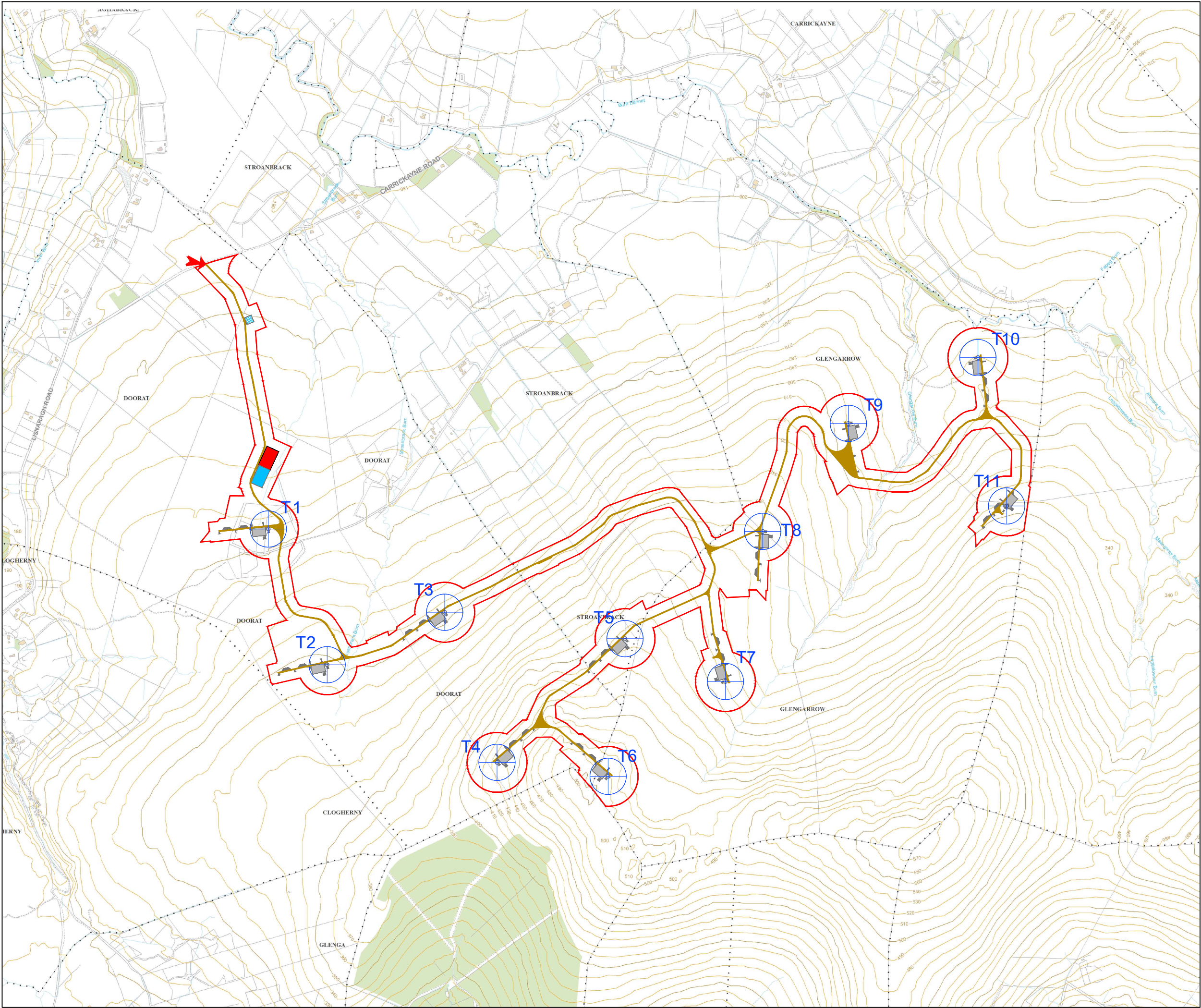
FIGURE 1.3 INFRASTRUCTURE LAYOUT
